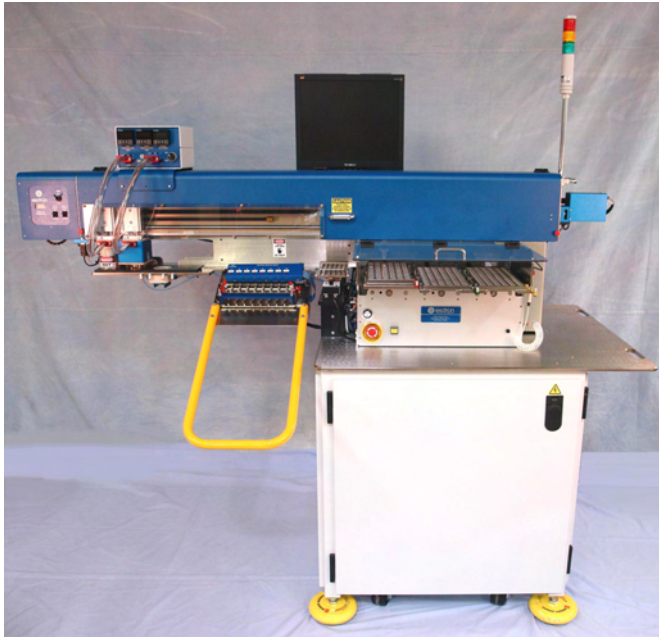
Tube/tray in/out with thermal test
