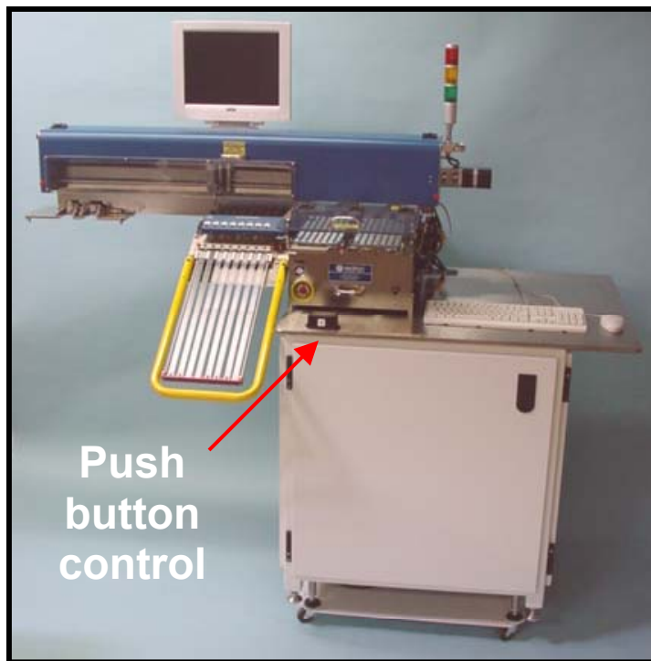
Model 902 with 8 output tube option Direct dock to Agilent 84000 Tester
