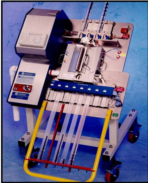
Wide sort 5000 for power devices 4 in-line high power test contactors
