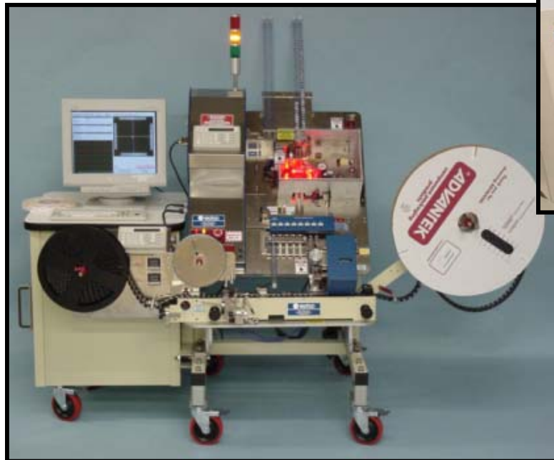
Model 5000 with 3D SOIC inspection and Model 1050 Tape & Reel output
