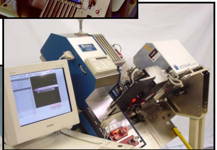
Custom 5000 with camera positioning system for precise laser cutting application
