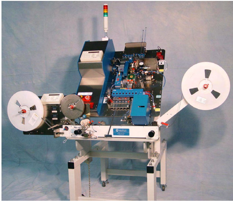
Model 5000 with taper output
