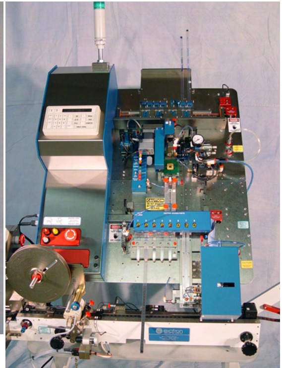
Model 5000 with taper output
