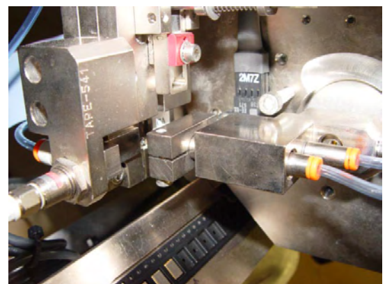
Taper swing arm getting device from output staging
