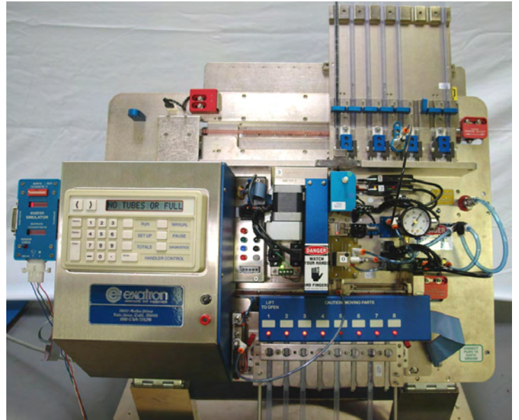
Gravity-feed with optional pickup head from index to test site to shuttle
