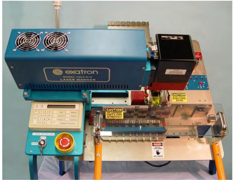
Laser marker integrated (Model L4)
