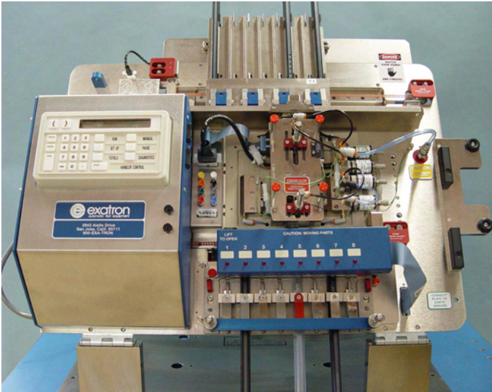
Straight gravity-feed
